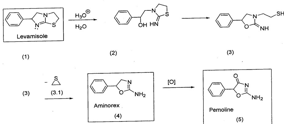
Figure 1: Postulated mechanism for the conversion of Levamisole into Aminorex into Pemoline. Under aqueous conditions Levamisole 1 can be protonated by \text{H}_3\text{O}^+ to form intermediate 2. The secondary alcohol in 2 can alkylate the double bond to form the neutral epoxide 3. The sulfur itself can be the possible nucleophile to lose the thiirane 3.1 to form Aminorex 4. It is known that Aminorex can undergo biological oxidation [\text{O}] to form Pemoline 5. [Eisenberg [2008], Ho, 2009].
